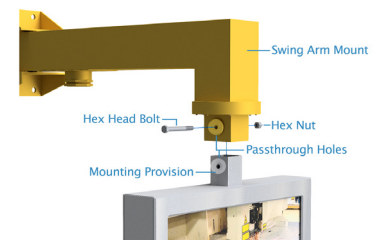
Swing arm/swivel
