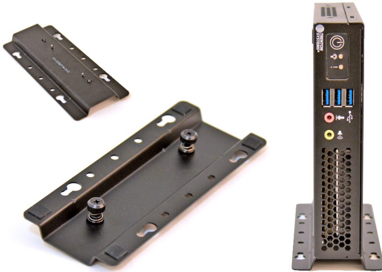
One-piece bracket P/N: 19850002114-00
